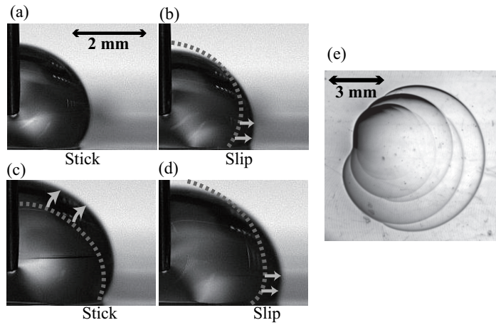
FIG. 2: (a)-(d) Sequential pictures of water droplet being inflated on SBS-paraffin gel ( c_{SBS} = 10\% ) at an inflation rate q = 20 \mu\text{l}/\text{min} . In images (b)-(d), a contour line of the previous droplet shape is drawn as a dotted line. During the inflation process, the contact line shows stick-slip behavior, i.e., the contact is fixed during a certain moment, then quickly advances. (e) A picture of the gel surface taken after the inflation process is finished and the droplet is removed. The droplet leaves multiple circular patterns.
