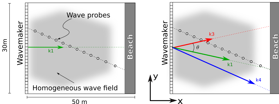
FIG. 1. Experimental setup for a 1D wave forcing (left, Secs. III and IV) and 2D bichromatic one (Sec. V).
