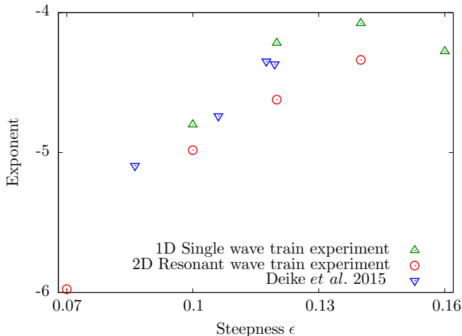
FIG. 9. Exponent of the frequency-power law spectrum of the wave energy as a function of the wave steepness \epsilon for the 1D single noisy wave-train experiment (1D NWT Sec. IV), the 2D resonant wave train experiment (2D RWT Sec. V), and the experiments of Deike et al. [27] in the configuration with a beach. These data correspond to x = 7.05 m (1D NWT) and x = 7.4 m (2D RWT and Ref. [27]).
