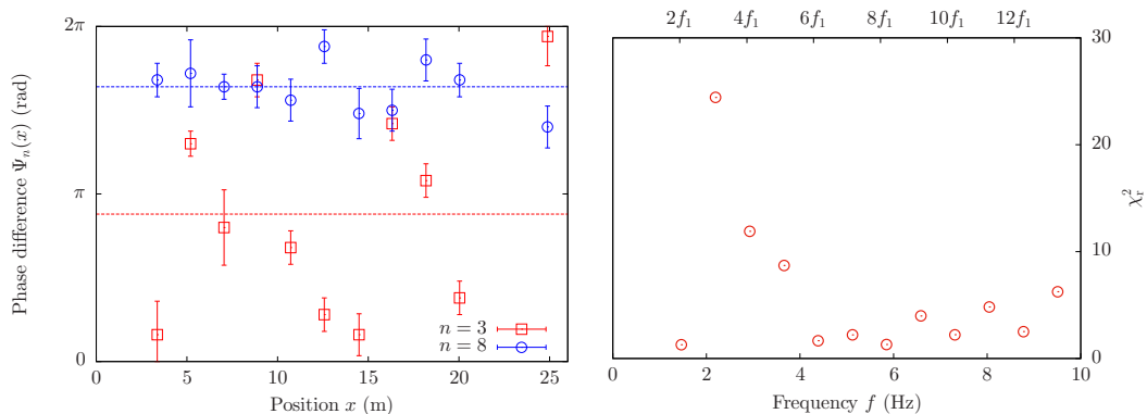
FIG. 3. Left: Evolution of the phase difference \Psi_n with the distance x to the wave maker for n = 3 and n = 8 . The two fits by constant functions are also reported (dashed lines). Right: coefficients \chi_r^2 computed for the constant fits on \Psi_n(x) .
