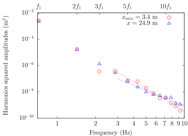
FIG. 4. Experimental evolution of the harmonic amplitudes, for n = 1 to 13 and for two distances from the wave maker x . The forcing is 1D and monochromatic ( f_1 = 0.715 Hz). Dashed lines are power laws of the form f^{-5.6} and f^{-3.9} .
