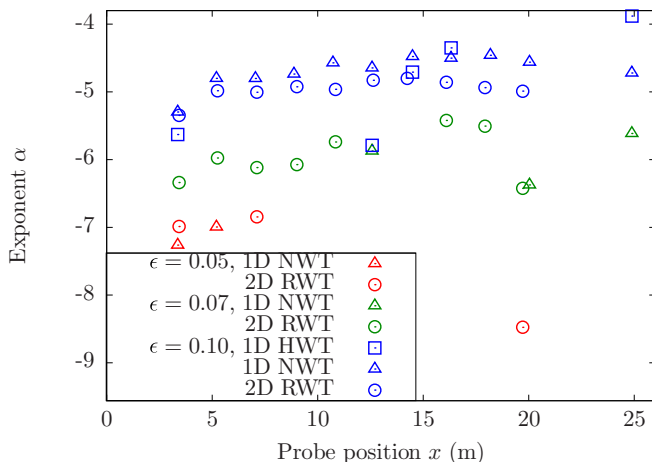
FIG. 6. Exponent \alpha of the energy spectrum in f^\alpha as a function of the distance from the wave maker, for three steepnesses \epsilon = \{0.05, 0.07, 0.10\} . ( \square ) Refer to a harmonic forcing (HWT, described in Sec. III), ( \triangle ) refer to a noisy wave train regardless of \Delta f (NWT, described in Sec. IV), and ( \circ ) refer to two wave trains in resonant interaction (RWT, described in Sec. V).
