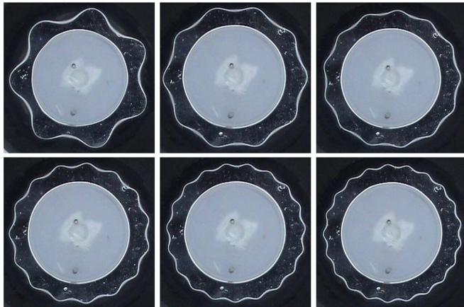
Top view of the pattern observed on the outer periphery of a mercury ring subjected to vibrations. The number of lobes increases with the frequency of the vibration (respectively from left to right, from top to bottom). The gray area corresponds to the central solid cylinder. Diameter of the torus ~ 4 cm. Credit: Laroche et al.
